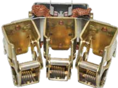
Roller Holders
